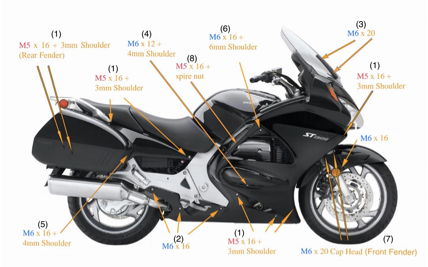
Diagram for Bolt Locations (on either side)
